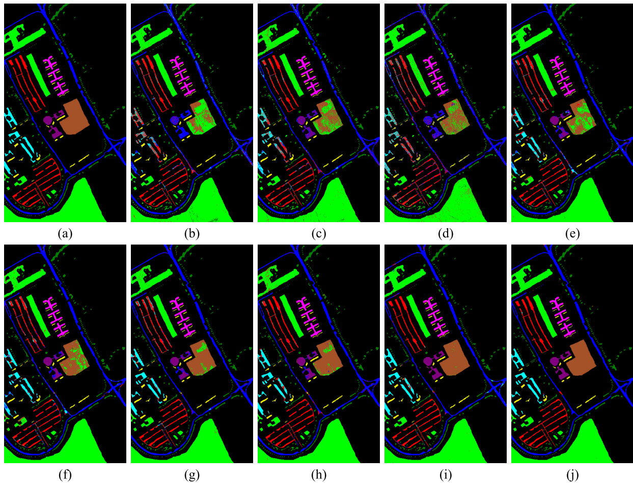
Fig. 12. Classification maps of the Pavia University dataset. (a) Ground-truth map. (b) SVM (OA = 82.76%). (c) EMAP (OA = 84.89%). (d) 1-D-CNN (OA = 83.50%). (e) 2-D-CNN (OA = 90.19%). (f) 3-D-CNN (OA = 92.01%). (g) SSRN (OA = 95.87%). (h) Cubic-CNN (OA = 95.68%). (i) HybridSN (OA = 98.16%). (j) SSFTT (OA = 99.21%).
