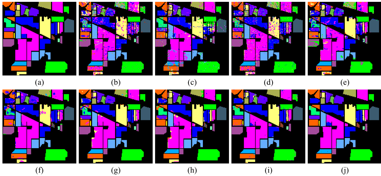
Fig. 11. Classification maps of the Indian Pines dataset. (a) Ground-truth map. (b) SVM (OA = 76.39%). (c) EMAP (OA = 83.69%). (d) 1-D-CNN (OA = 79.37%). (e) 2-D-CNN (OA = 84.47%). (f) 3-D-CNN (OA = 91.03%). (g) SSRN (OA = 94.78%). (h) Cubic-CNN (OA = 94.90%). (i) HybridSN (OA = 96.62%). (j) SSFTT (OA = 97.47%).
